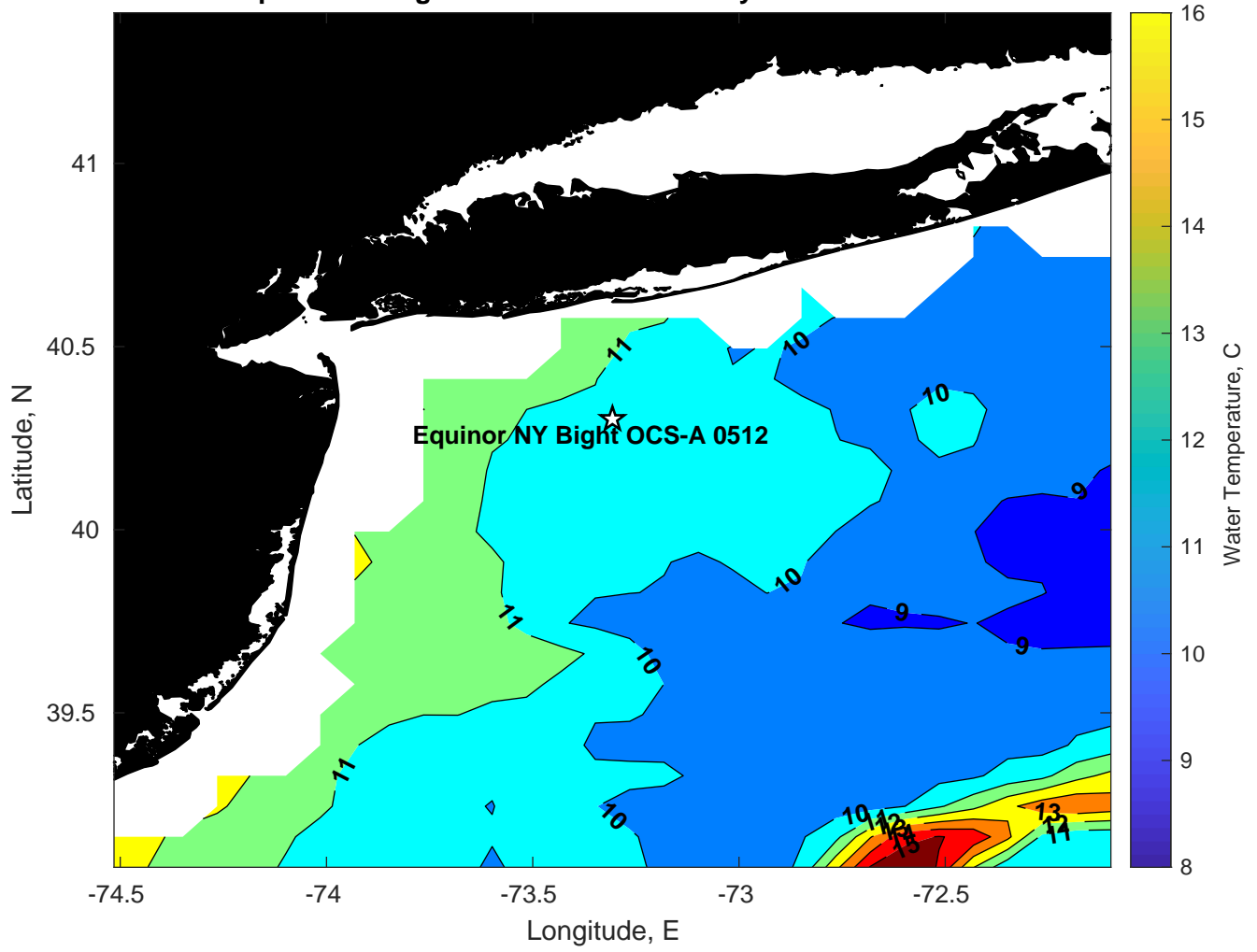
SST for Equinor NY Bight OCS-A 0512 at 04-May-2024 00:00:00
